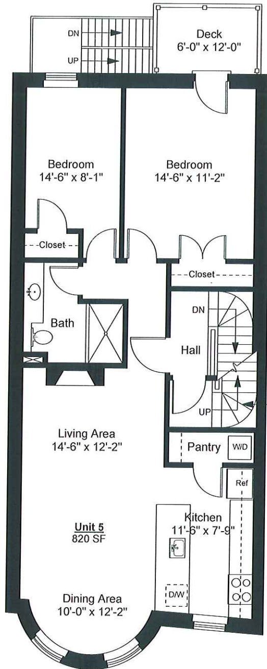
Unit 5 Floor Plan
