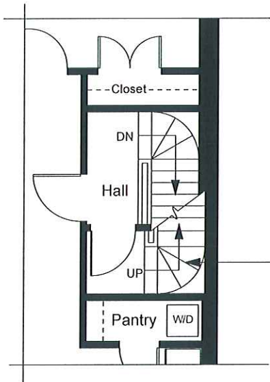
Unit 6 Entry Detail Plan
