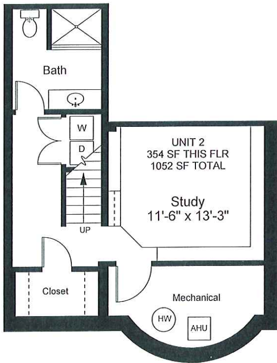
Unit 2 Garden Level Floor Plan
