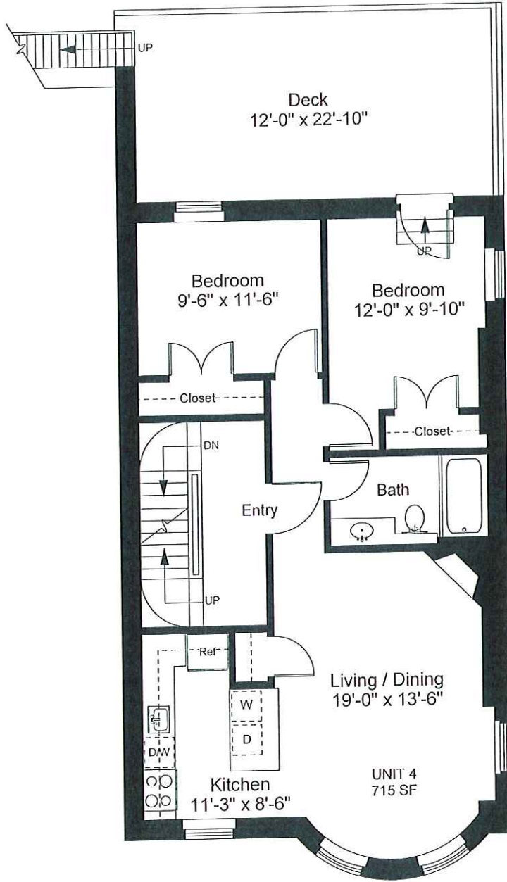
Unit 4 Floor Plan
